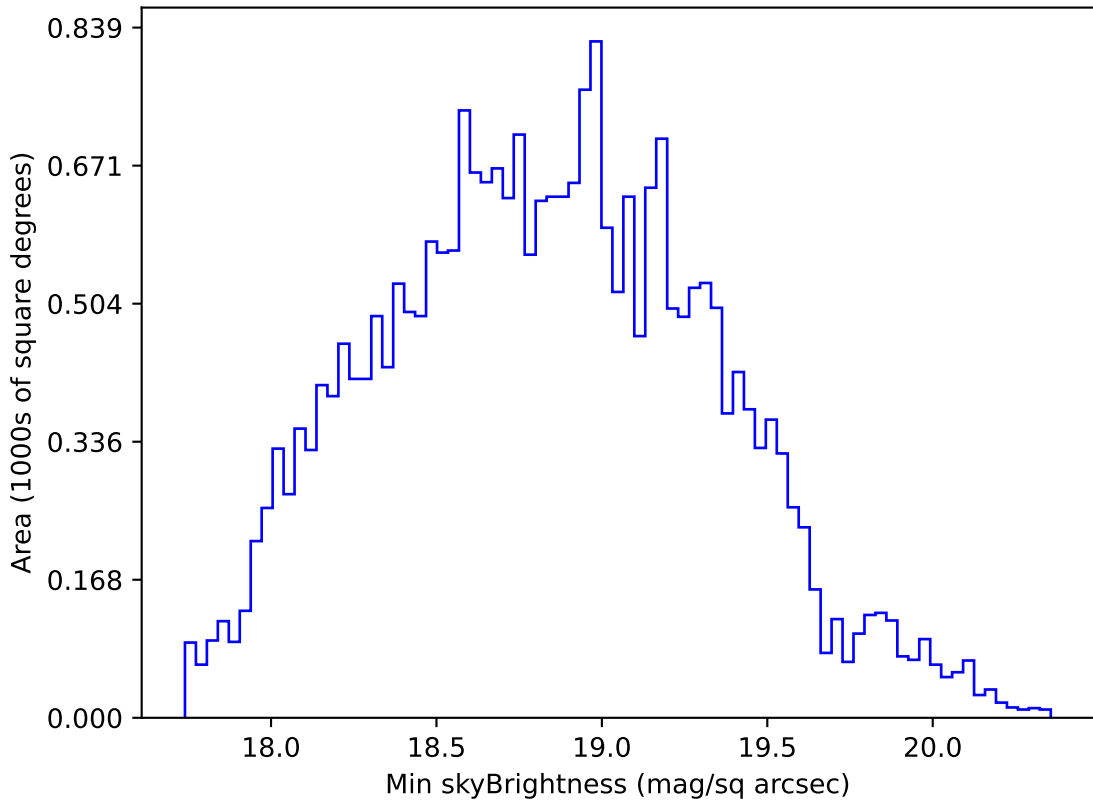
ddf_acor_sf10_lsf30_lsr10_v3.4_10yrs All sky r band: Min skyBrightness
