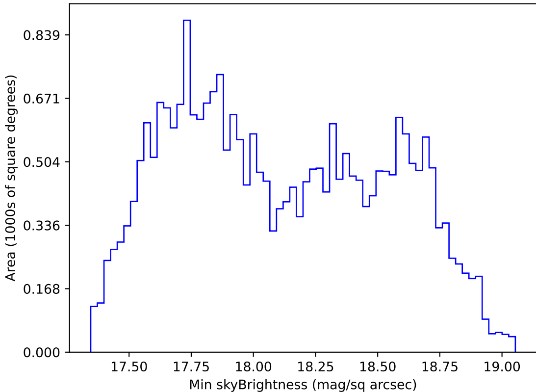
ddf_acor_sf10_ls30_lsr10_v3.4_10yrs All sky i band: Min skyBrightness
