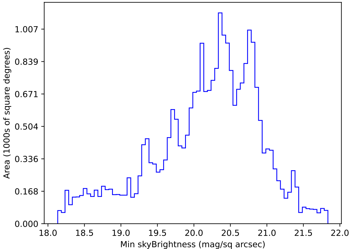
ddf_acor_sf10_lsf30_lsr10_v3.4_10yrs All sky g band: Min skyBrightness
