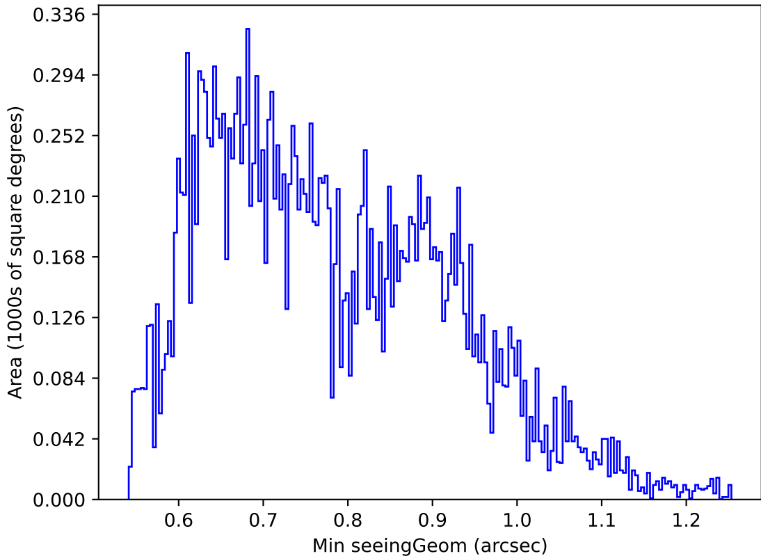
ddf_acor_sf10_ls30_lsr10_v3.4_10yrs Yr 1 u band: Min seeingGeom
