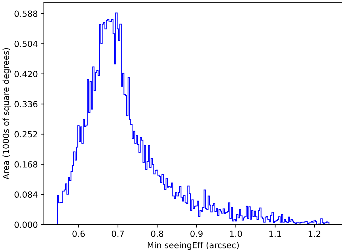
ddf_acor_sf10_lsf30_lsr10_v3.4_10yrs Yr 1 z band: Min seeingEff
