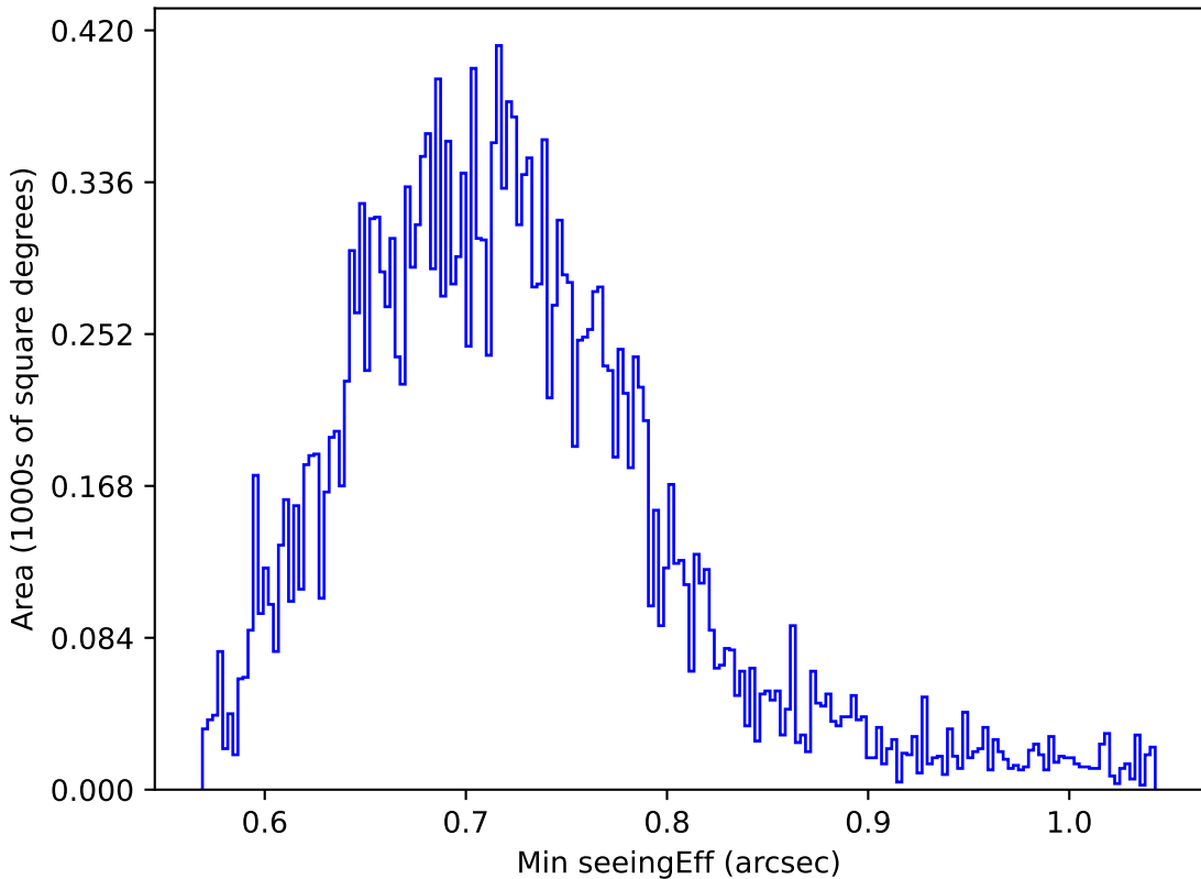
ddf_acor_sf10_lsf30_lsr10_v3.4_10yrs Yr 1 y band: Min seeingEff
