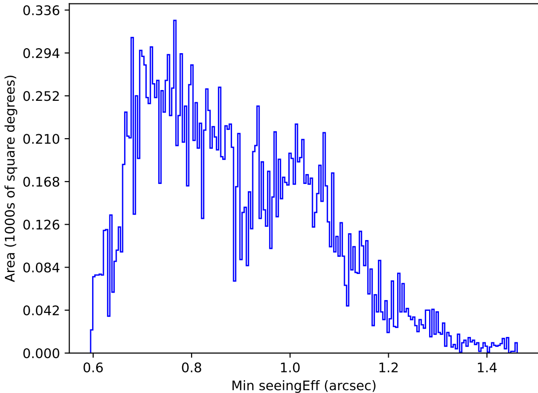
ddf_acor_sf10_lsf30_lsr10_v3.4_10yrs Yr 1 u band: Min seeingEff
