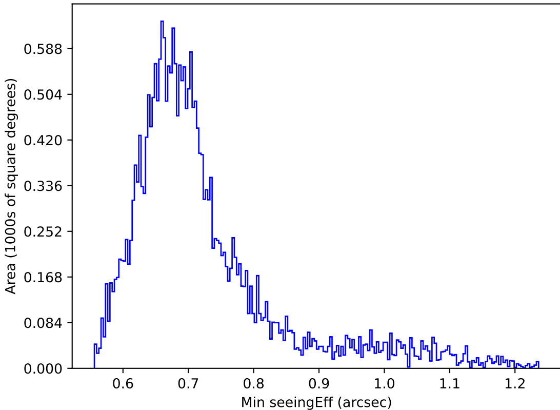
ddf_acor_sf10_ls30_lsr10_v3.4_10yrs Yr 1 r band: Min seeingEff
