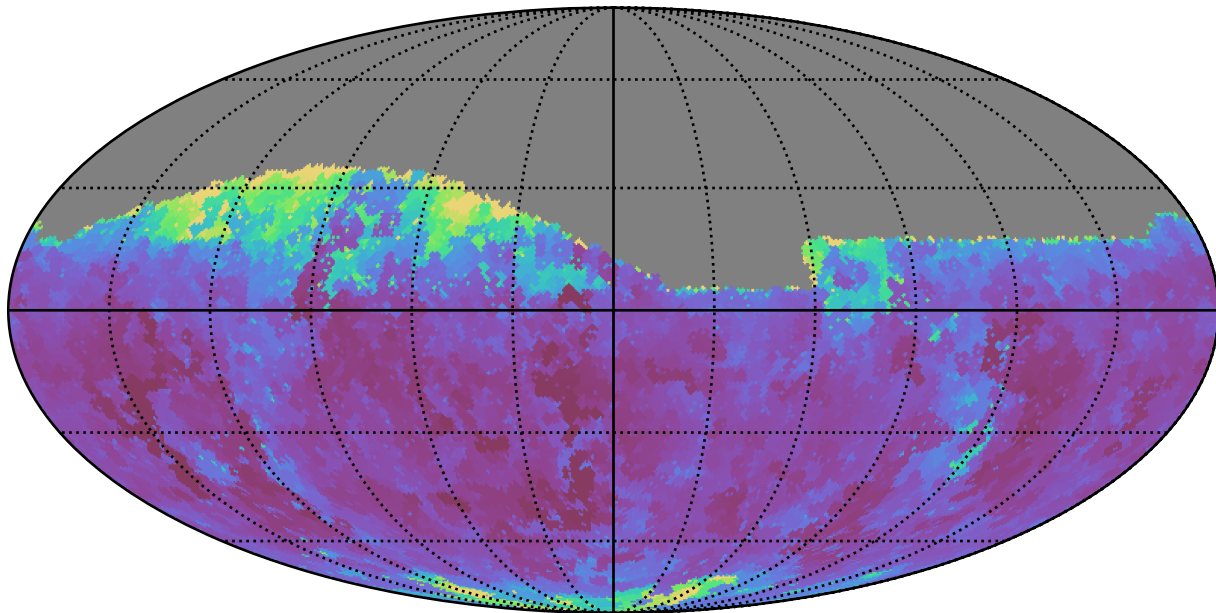
ddf_acor_sf10_lsf30_lsr10_v3.4_10yrs Yr 1 i band: Min seeingEff
