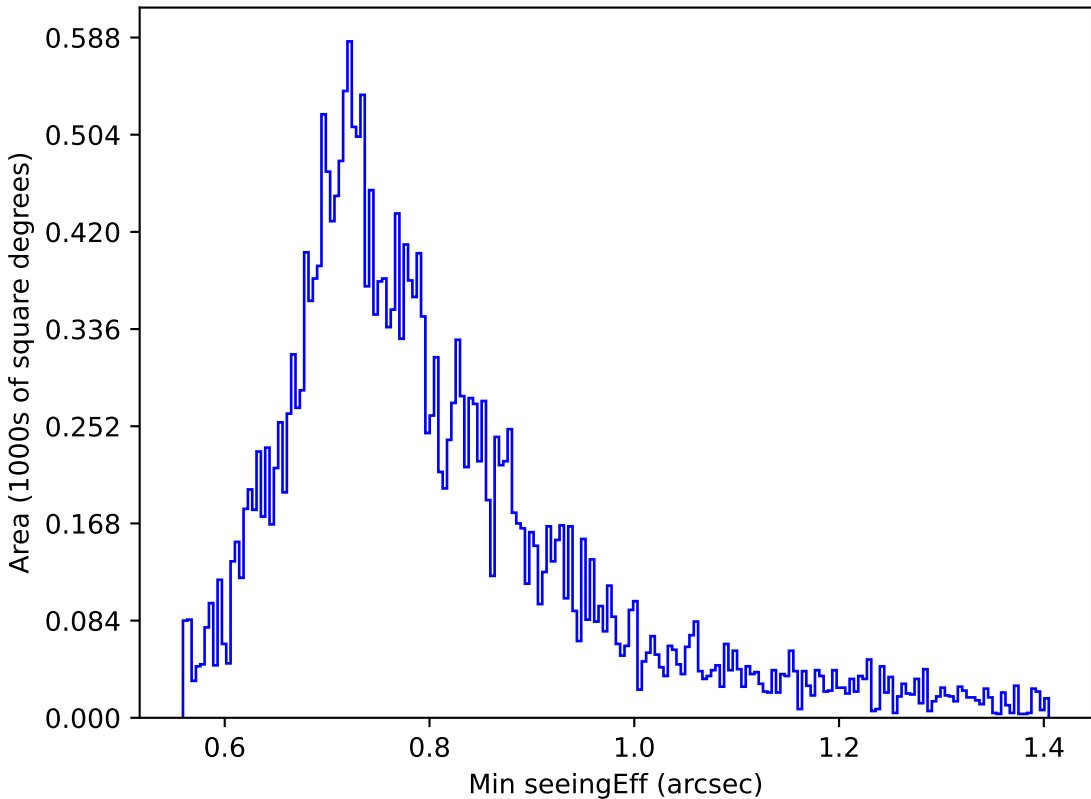
ddf_acor_sf10_lsf30_lsr10_v3.4_10yrs Yr 1 g band: Min seeingEff
