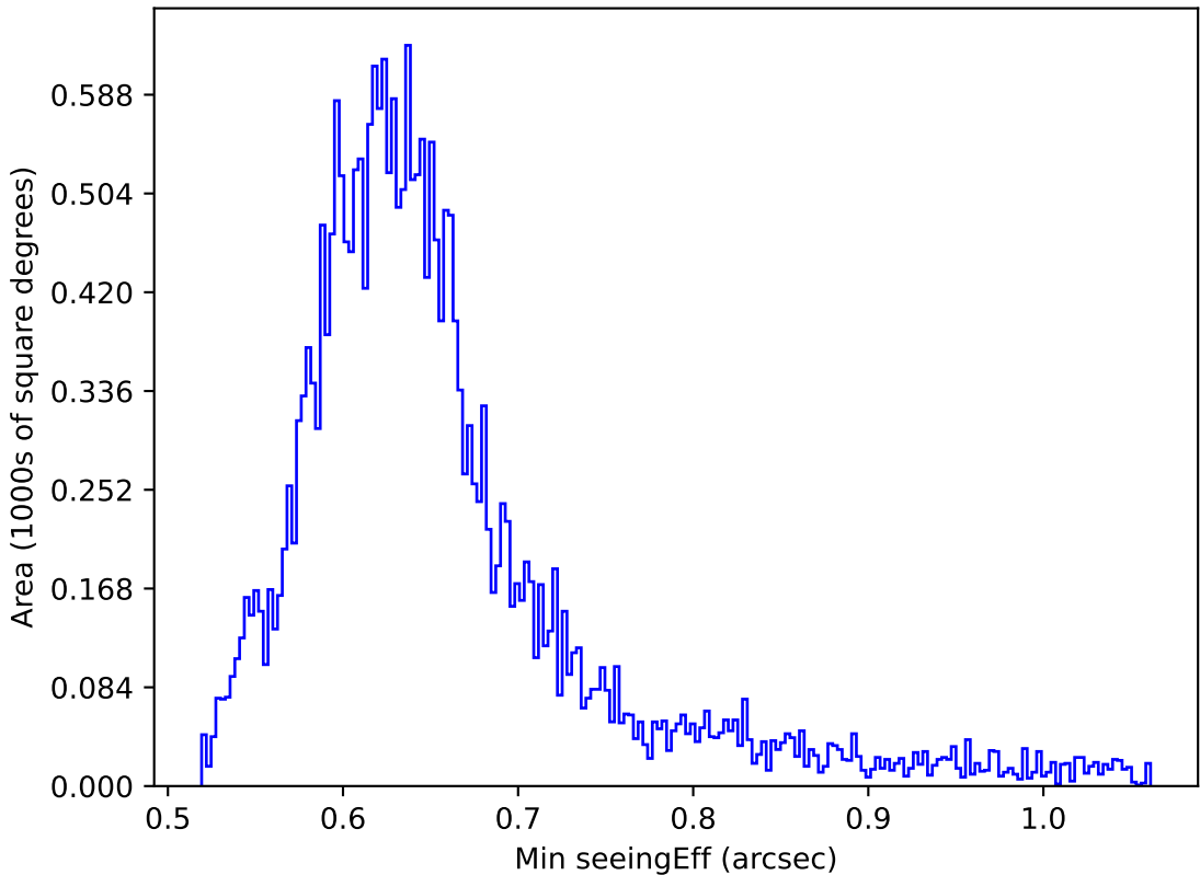
ddf_acor_sf10_lsf30_lsr10_v3.4_10yrs Yr 1 all bands: Min seeingEff
