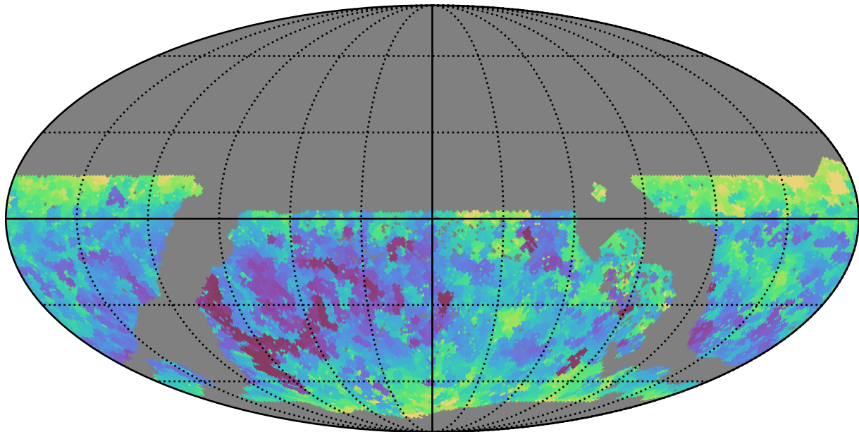
ddf_acor_sf10_lsf30_lsr10_v3.4_10yrs WFD y band: Min seeingEff
