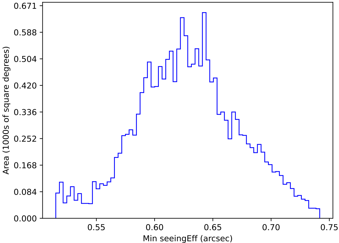
ddf_acor_sf10_lsf30_lsr10_v3.4_10yrs WFD y band: Min seeingEff
