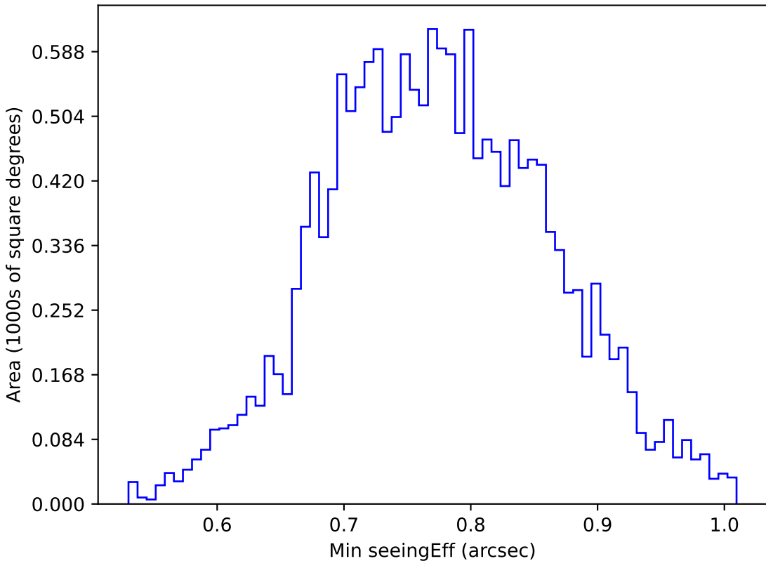
ddf_acor_sf10_lsf30_lsr10_v3.4_10yrs WFD u band: Min seeingEff
