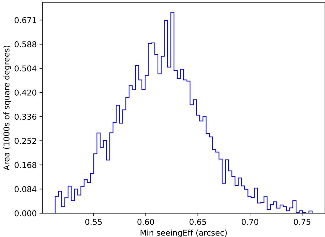
ddf_acor_sf10_lsf30_lsr10_v3.4_10yrs WFD r band: Min seeingEff
