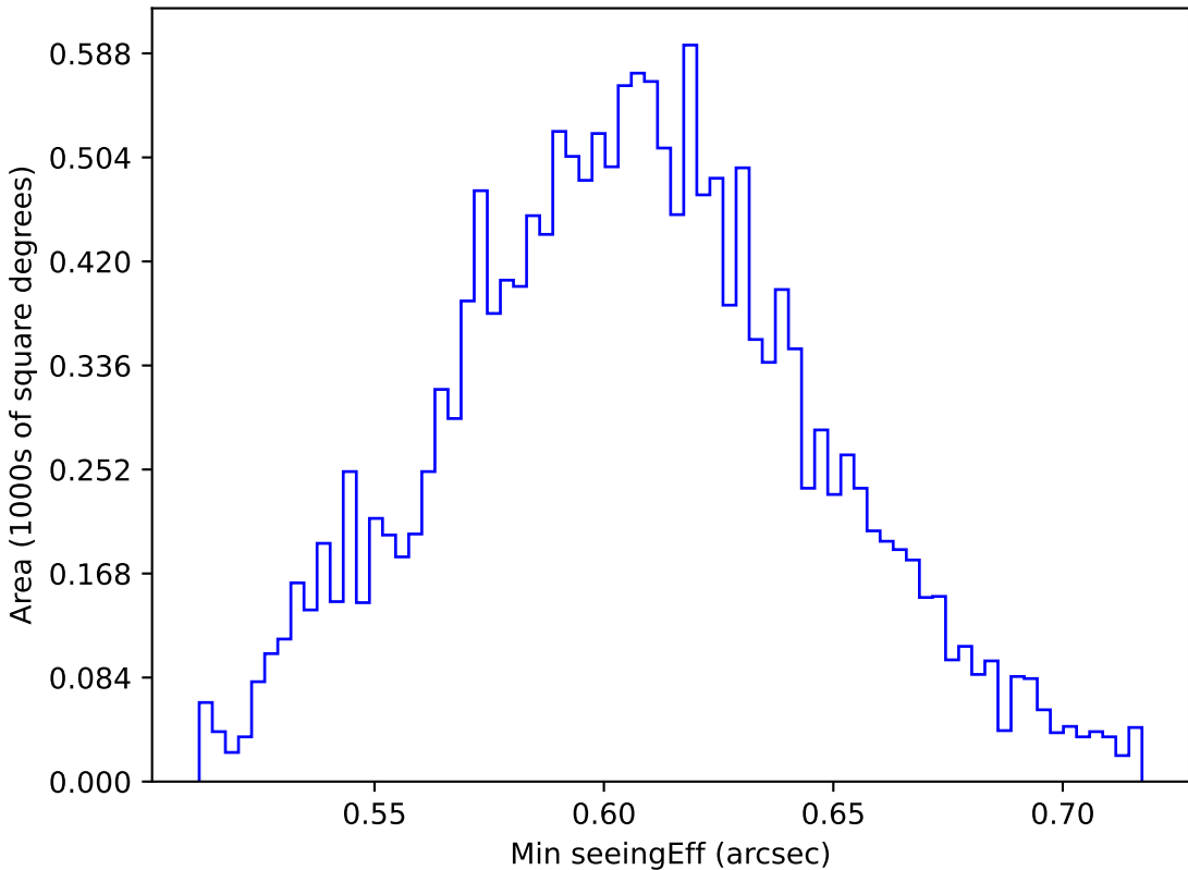
ddf_acor_sf10_lsf30_lsr10_v3.4_10yrs WFD i band: Min seeingEff
