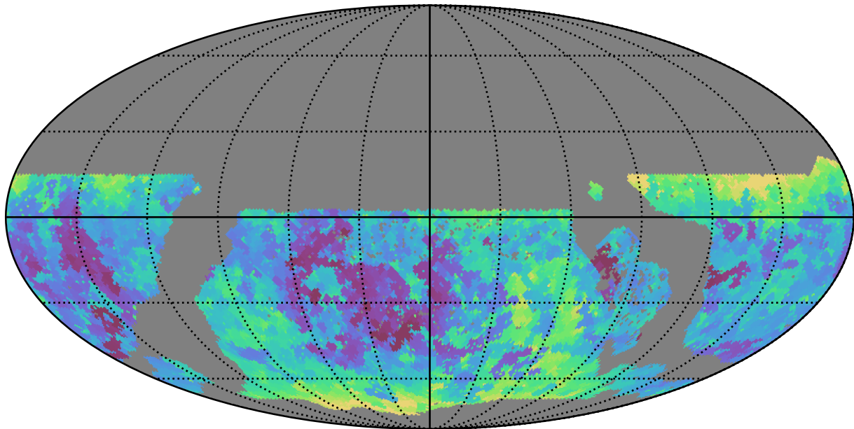
ddf_acor_sf10_lsf30_lsr10_v3.4_10yrs WFD g band: Min seeingEff
