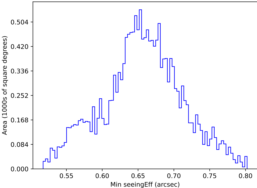
ddf_acor_sf10_lsf30_lsr10_v3.4_10yrs WFD g band: Min seeingEff
