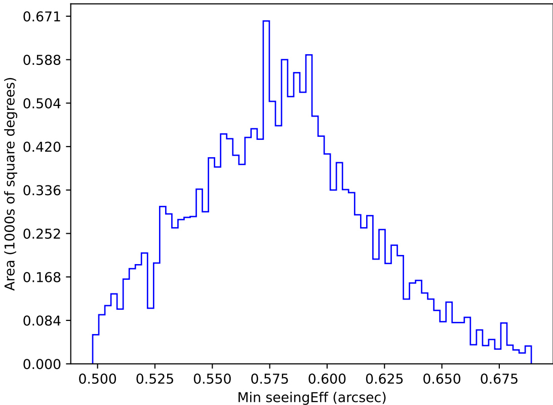
ddf_acor_sf10_lsf30_lsr10_v3.4_10yrs WFD all bands: Min seeingEff
