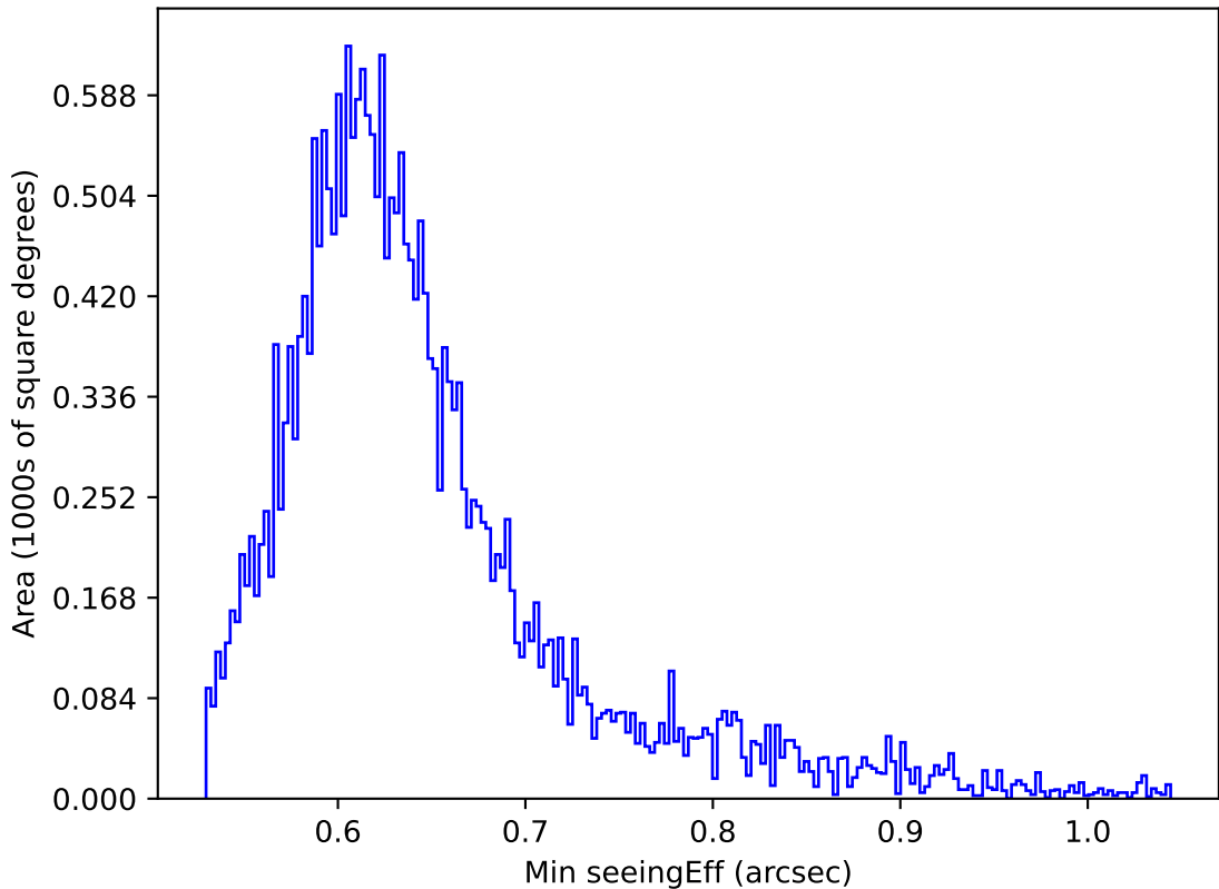
ddf_acor_sf10_lsf30_lsr10_v3.4_10yrs All sky z band: Min seeingEff
