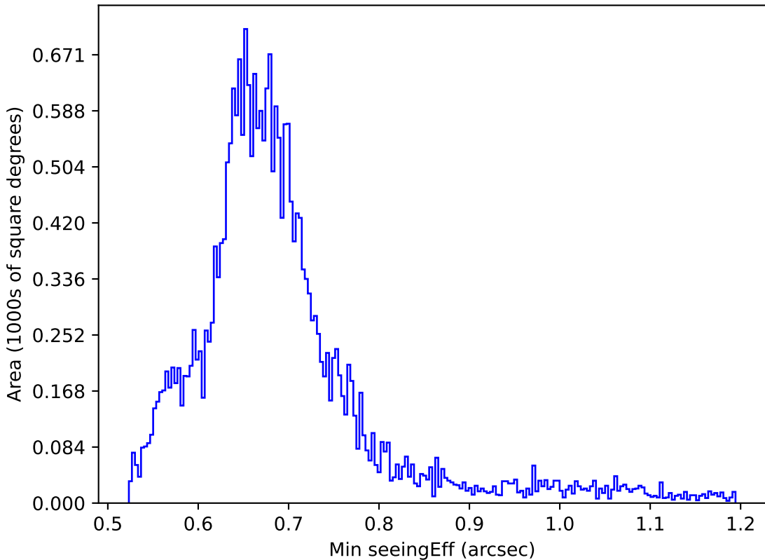
ddf_acor_sf10_lsf30_lsr10_v3.4_10yrs All sky g band: Min seeingEff
