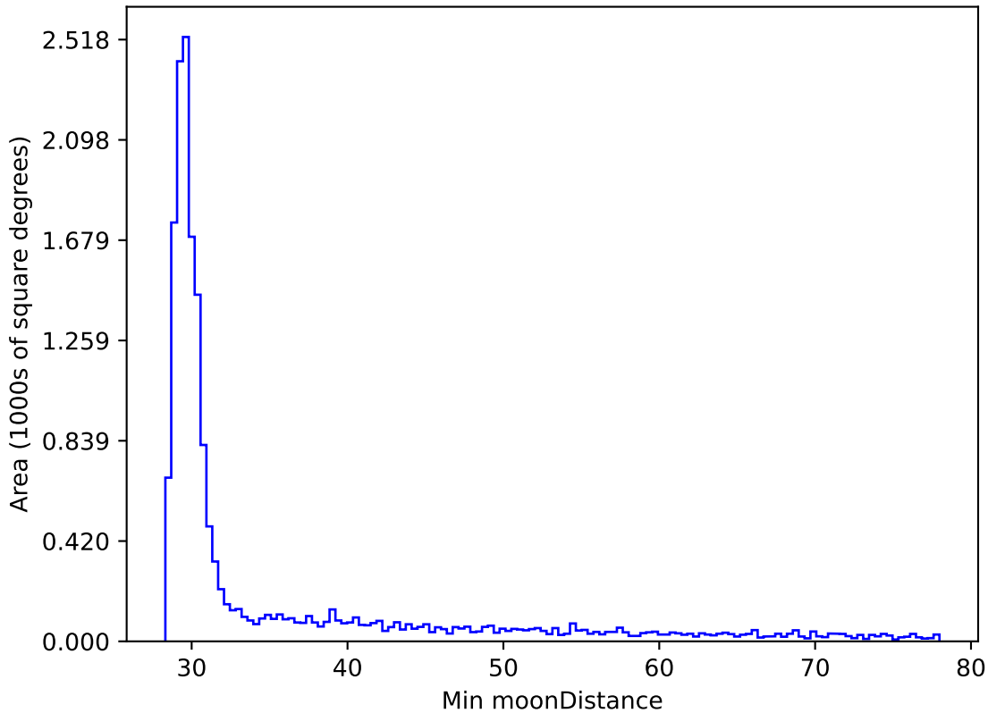
ddf_acor_sf10_lsf30_lsr10_v3.4_10yrs WFD z band: Min moonDistance
