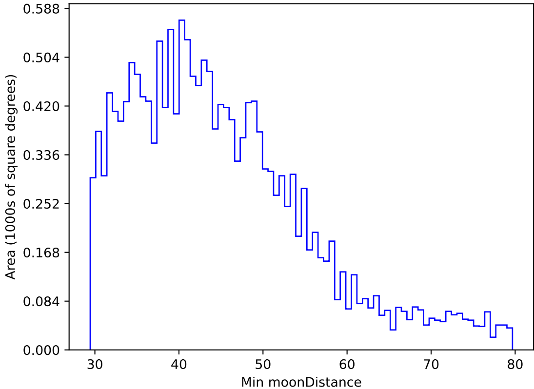
ddf_acor_sf10_lsf30_lsr10_v3.4_10yrs WFD g band: Min moonDistance
