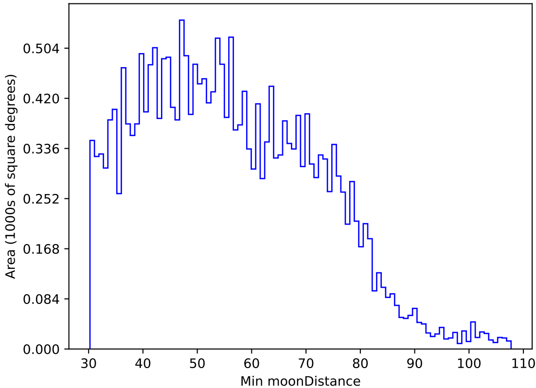
ddf_acor_sf10_lsf30_lsr10_v3.4_10yrs All sky u band: Min moonDistance
