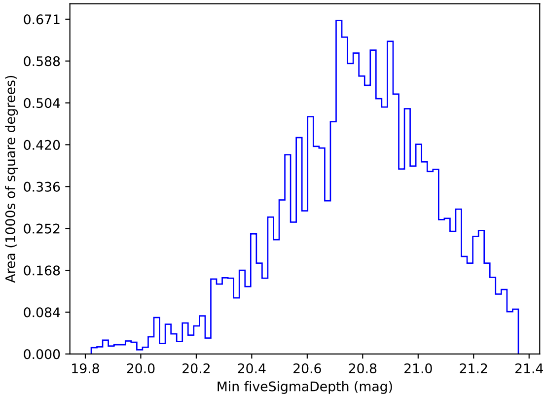
ddf_acor_sf10_lsf30_lsr10_v3.4_10yrs WFD all bands: Min fiveSigmaDepth
