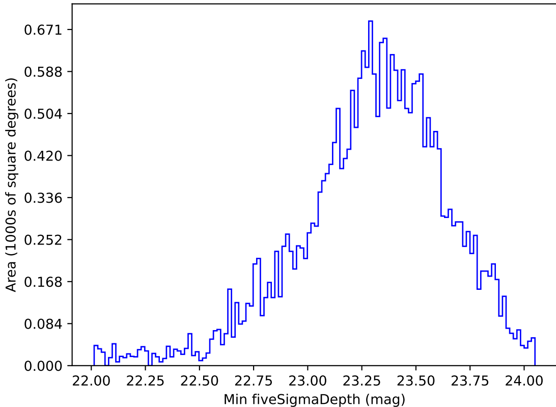
ddf_acor_sf10_lsf30_lsr10_v3.4_10yrs All sky g band: Min fiveSigmaDepth
