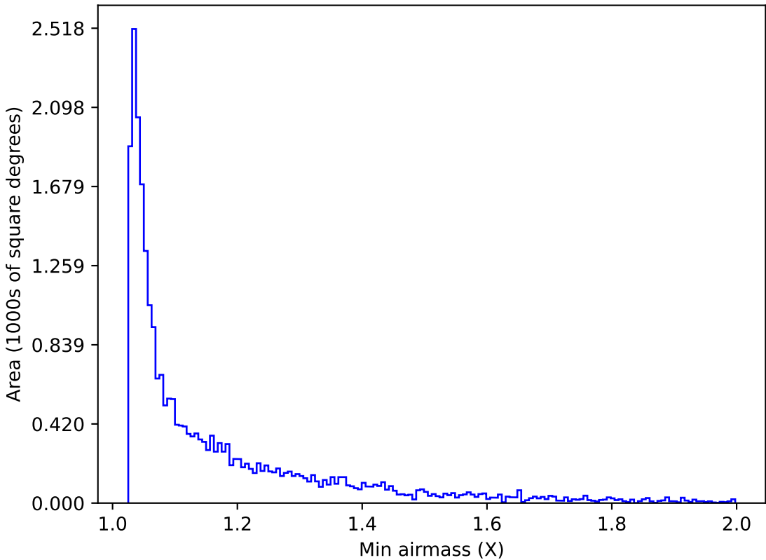
ddf_acor_sf10_lsf30_lsr10_v3.4_10yrs Yr 1 z band: Min airmass
