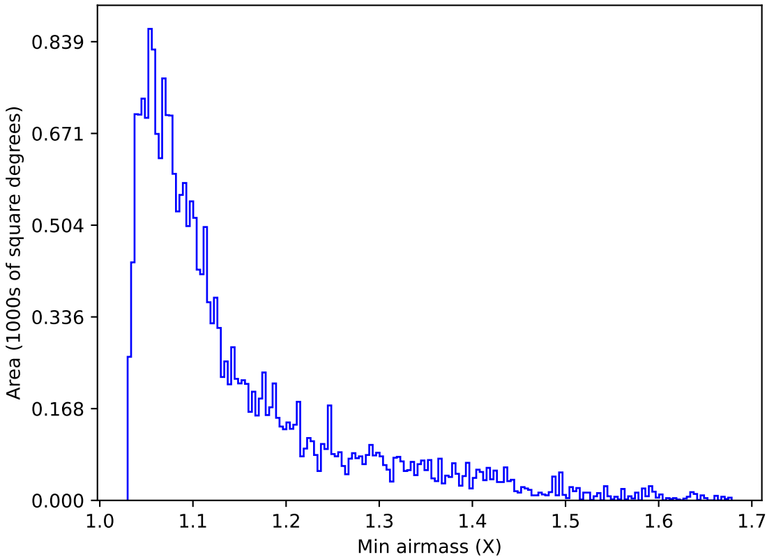
ddf_acor_sf10_lsf30_lsr10_v3.4_10yrs Yr 1 u band: Min airmass
