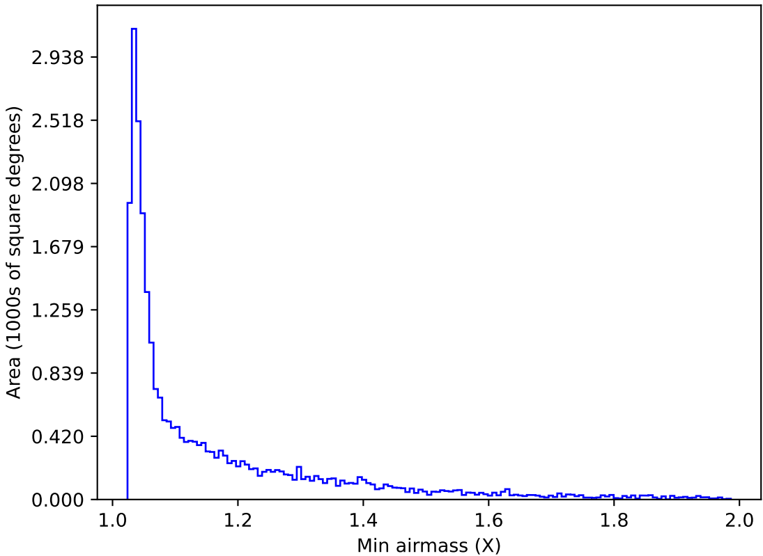
ddf_acor_sf10_lsf30_lsr10_v3.4_10yrs Yr 1 r band: Min airmass
