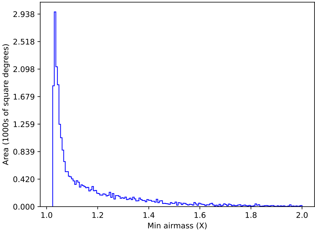
ddf_acor_sf10_lsf30_lsr10_v3.4_10yrs Yr 1 i band: Min airmass
