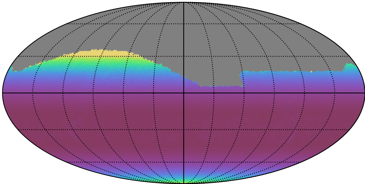
ddf_acor_sf10_lsf30_lsr10_v3.4_10yrs Yr 1 all bands: Min airmass
