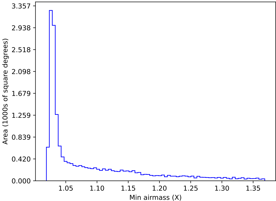
ddf_acor_sf10_lsf30_lsr10_v3.4_10yrs WFD z band: Min airmass
