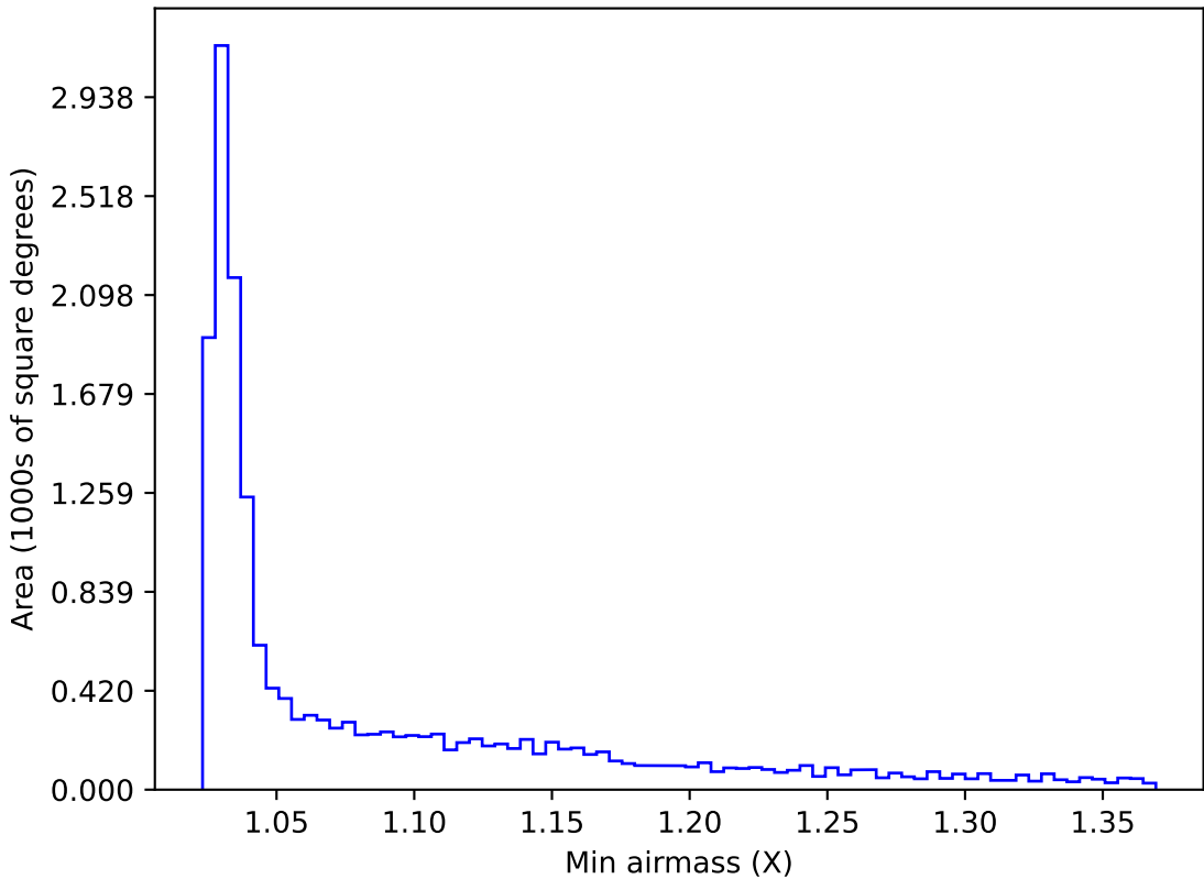
ddf_acor_sf10_lsf30_lsr10_v3.4_10yrs WFD y band: Min airmass
