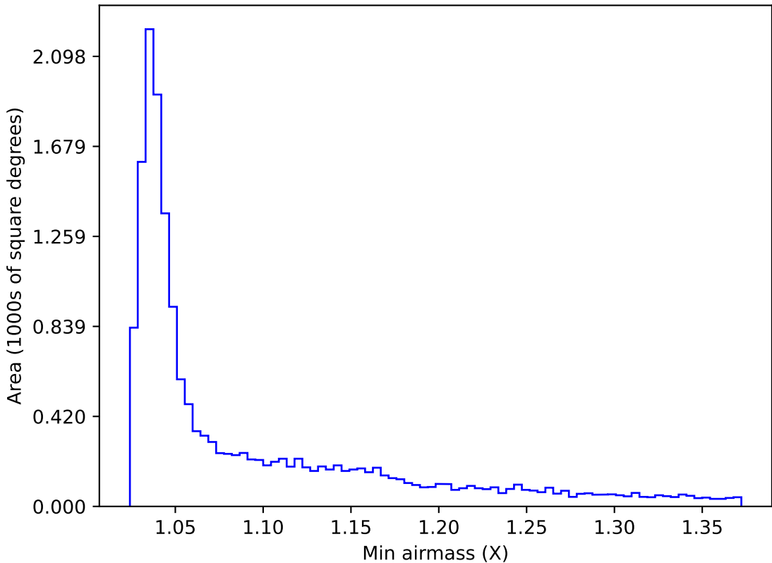
ddf_acor_sf10_lsf30_lsr10_v3.4_10yrs WFD u band: Min airmass
