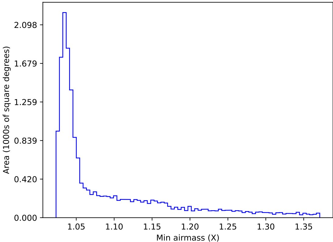
ddf_acor_sf10_lsf30_lsr10_v3.4_10yrs WFD g band: Min airmass
