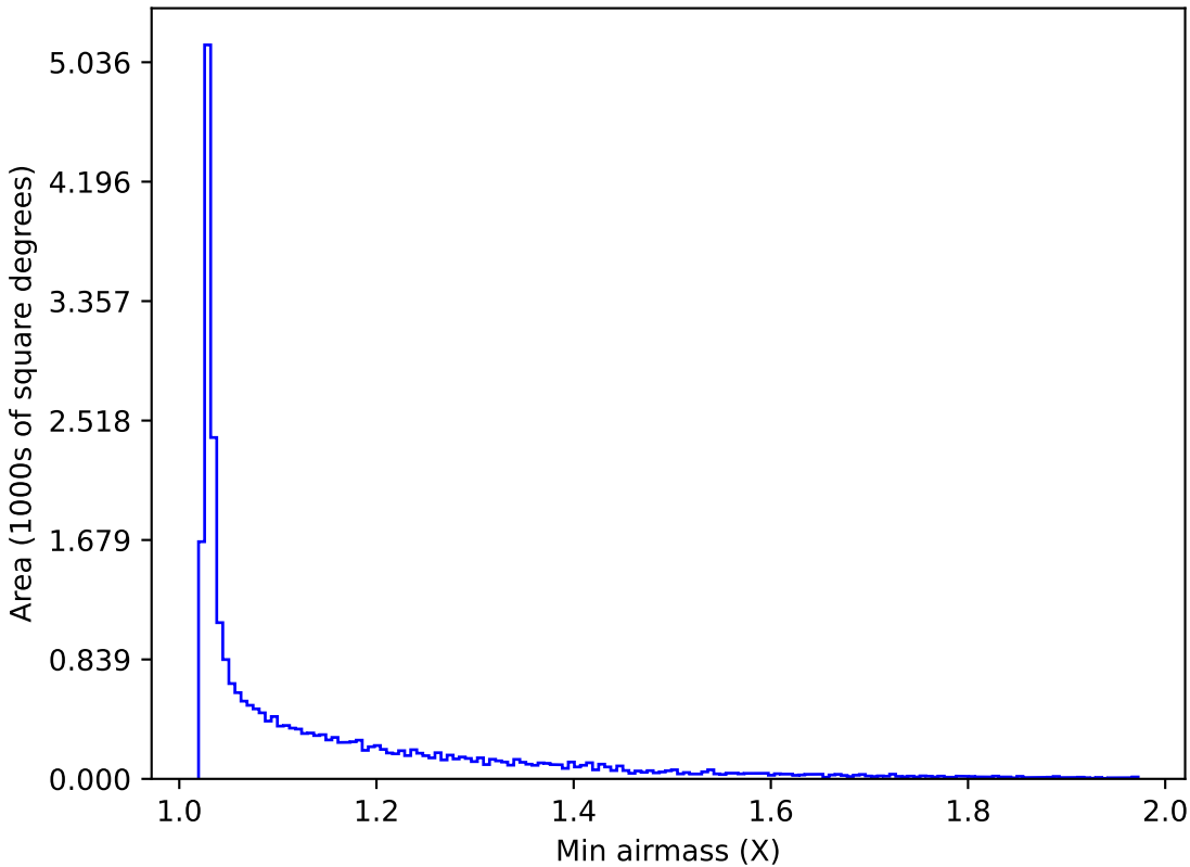
ddf_acor_sf10_lsf30_lsr10_v3.4_10yrs All sky z band: Min airmass
