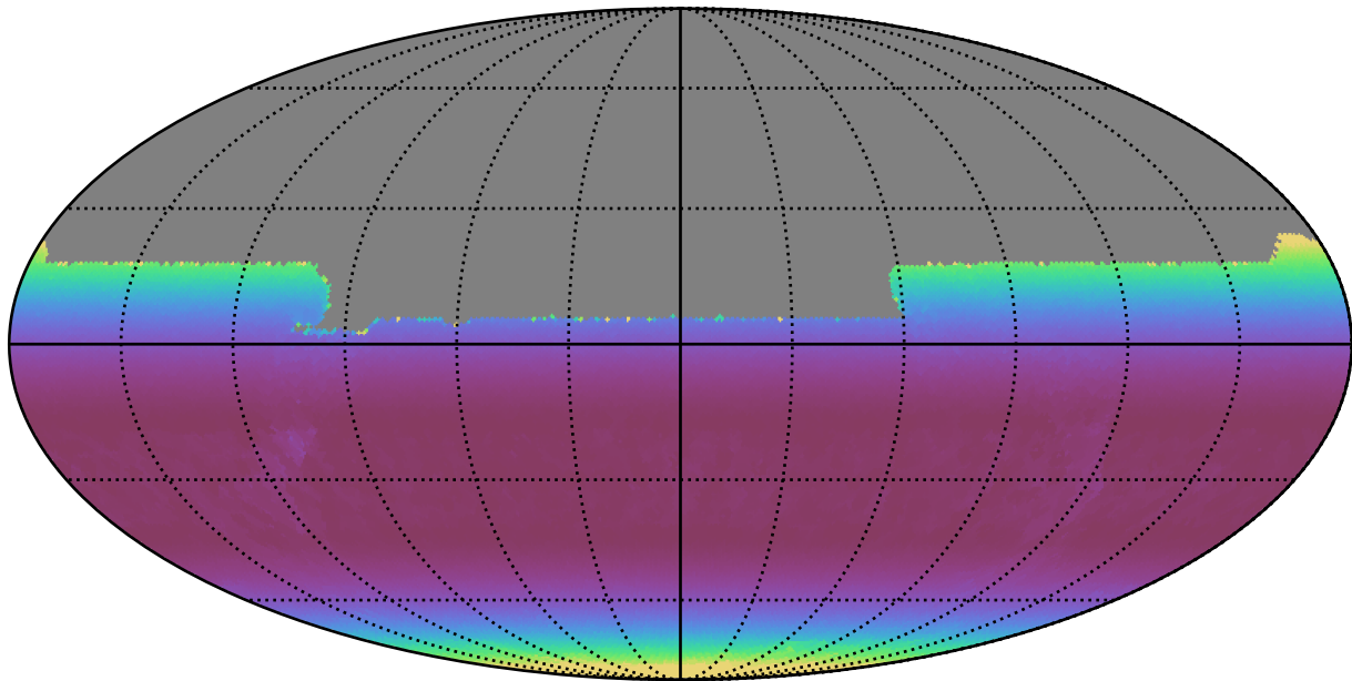
ddf_acor_sf10_lsf30_lsr10_v3.4_10yrs All sky y band: Min airmass
