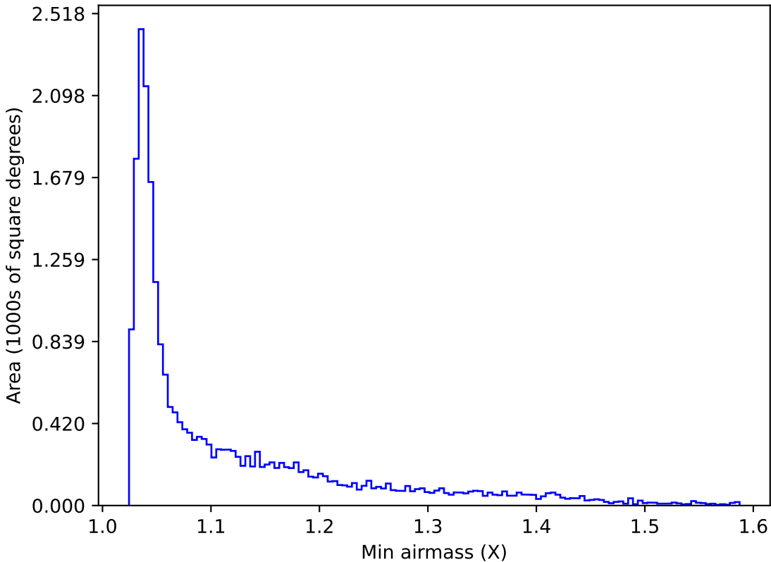
ddf_acor_sf10_lsf30_lsr10_v3.4_10yrs All sky u band: Min airmass
