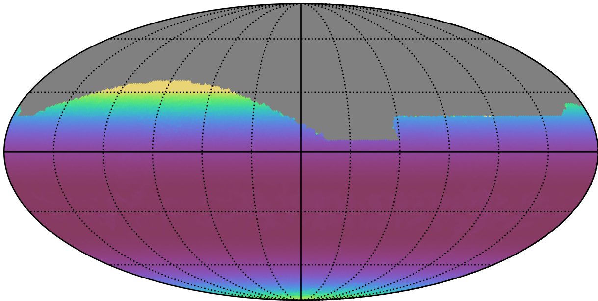
ddf_acor_sf10_lsf30_lsr10_v3.4_10yrs All sky r band: Min airmass
