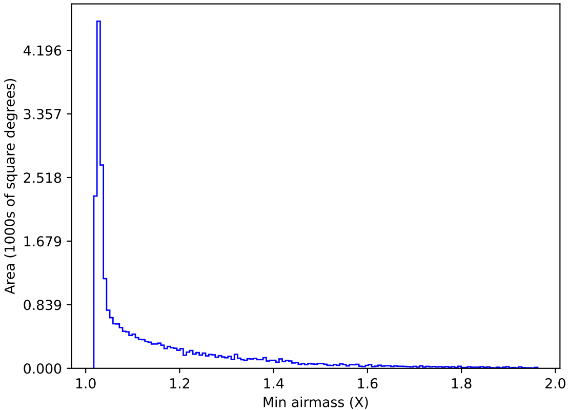
ddf_acor_sf10_lsf30_lsr10_v3.4_10yrs All sky r band: Min airmass
