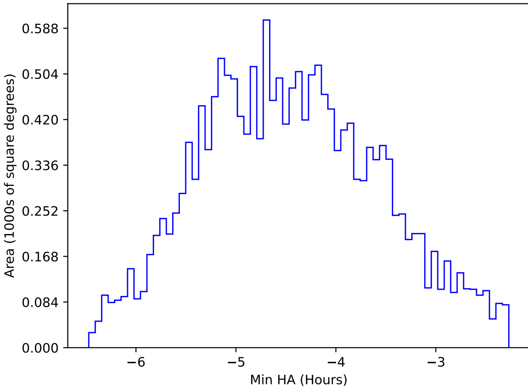
ddf_acor_sf10_lsf30_lsr10_v3.4_10yrs WFD r band: Min HA
