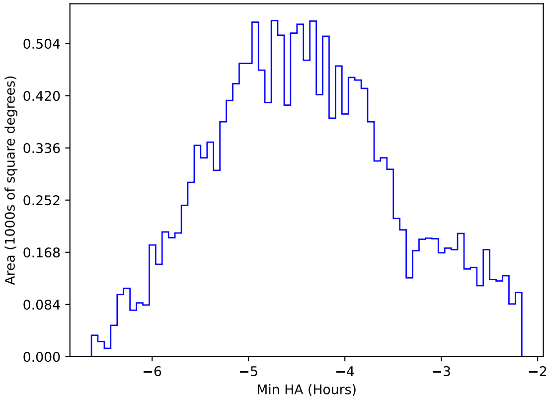
ddf_acor_sf10_lsf30_lsr10_v3.4_10yrs WFD i band: Min HA
