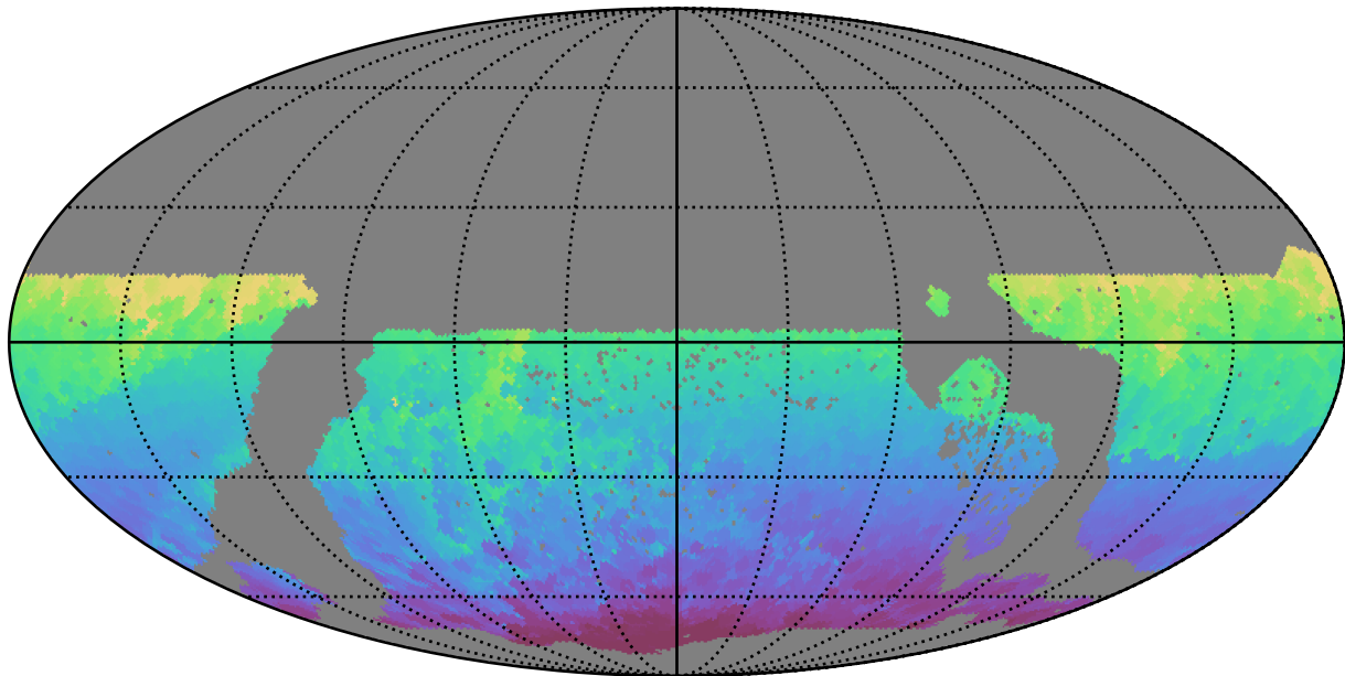
ddf_acor_sf10_lsf30_lsr10_v3.4_10yrs WFD all bands: Min HA
