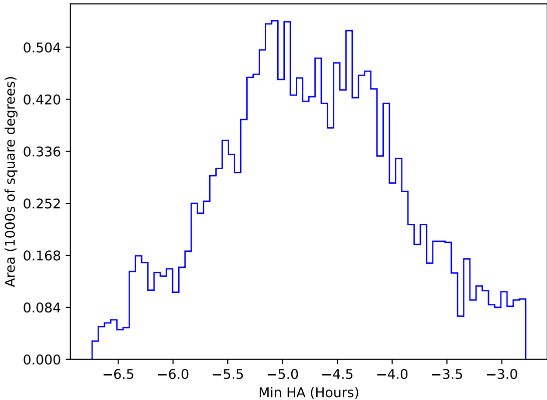
ddf_acor_sf10_ls30_lsr10_v3.4_10yrs WFD all bands: Min HA
