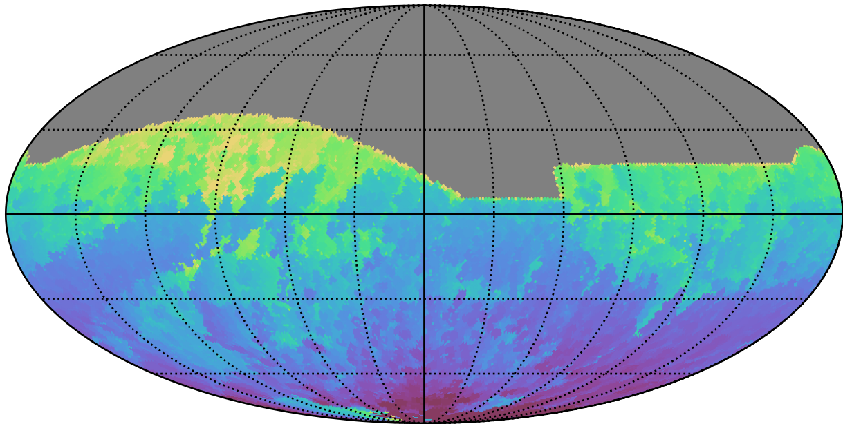
ddf_acor_sf10_lsf30_lsr10_v3.4_10yrs All sky z band: Min HA
