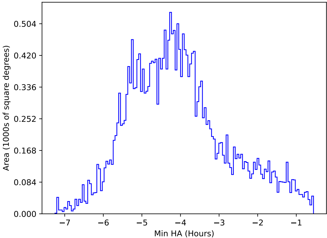
ddf_acor_sf10_lsf30_lsr10_v3.4_10yrs All sky z band: Min HA
