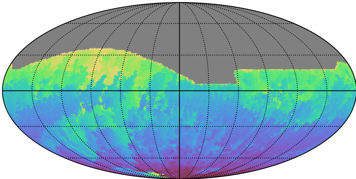
ddf_acor_sf10_lsf30_lsr10_v3.4_10yrs All sky i band: Min HA
