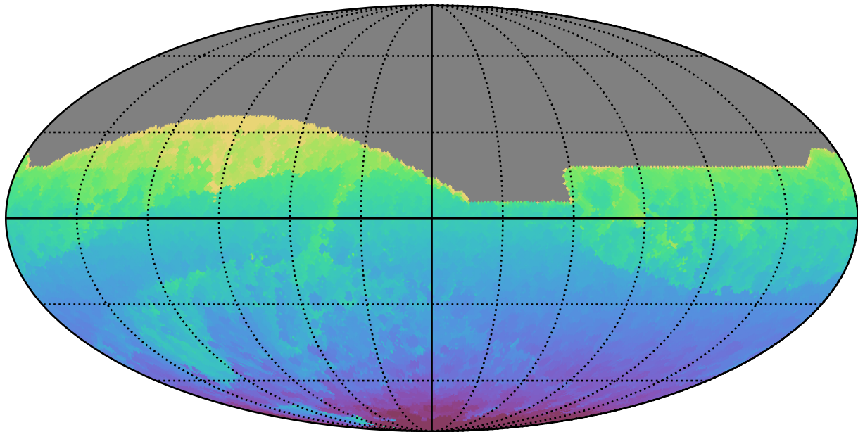
ddf_acor_sf10_lsf30_lsr10_v3.4_10yrs All sky all bands: Min HA
