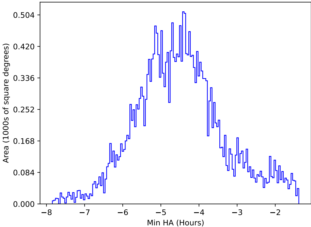
ddf_acor_sf10_lsf30_lsr10_v3.4_10yrs All sky all bands: Min HA
