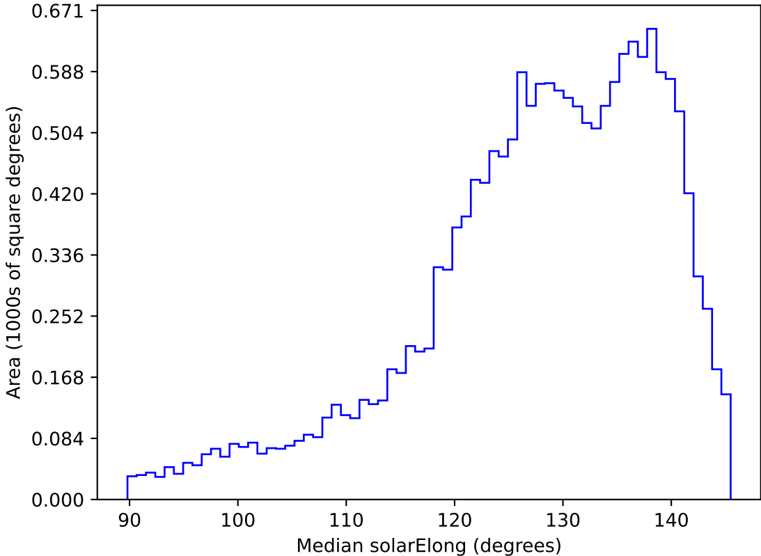
ddf_acor_sf10_lsf30_lsr10_v3.4_10yrs WFD z band: Median solarElong
